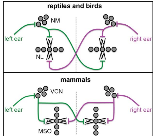
Figure 1. Schematic drawings of the organization of the binaural circuit in the reptilian, avian, and mammalian auditory brainstem. The reptilian and avian NM and NL are structurally and functionally similar to the mammalian VCN and MSO, respectively. The two dendritic domains of individual bipolar neurons in NL and MSO receive segregated excitatory inputs from the two ears. More specifically, cochlear ganglion cells provide excitatory input to the ipsilateral VCN in mammals and NM in reptiles and birds. Individual VCN and NM neurons project bilaterally to the segregated MSO and NL dendrites, respectively. In mammals, one collateral ends on the lateral dendrites and the cell body of the ipsilateral MSO neurons with the other collateral projecting to the medial dendrite and the cell body of the contralateral MSO. In birds and presumably in reptiles, this pattern is preserved, with NM neurons projecting to the dorsal dendritic domain of the ipsilateral NL and the ventral domain of the contralateral NL. Dashed lines indicate the midline. Dorsal is up. NM, nucleus magnocellularis; NL, nucleus laminaris; VCN, ventral cochlear nucleus; MSO, medial superior olive.
